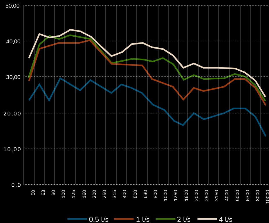
Measured airborne sound power level, L_{WA} [dB]
