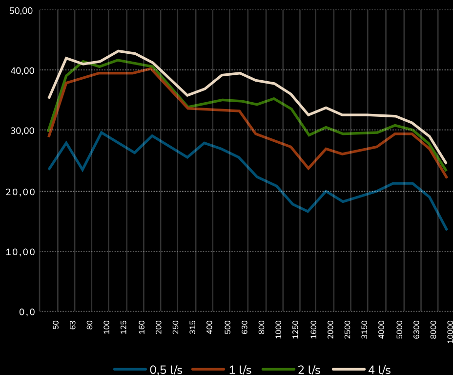
Airborne sound power level, L_{WA} [dB]
